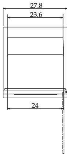
MUF-28 PLAN VIEW
