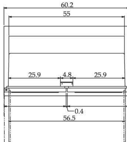
MUF-60 PLAN VIEW
