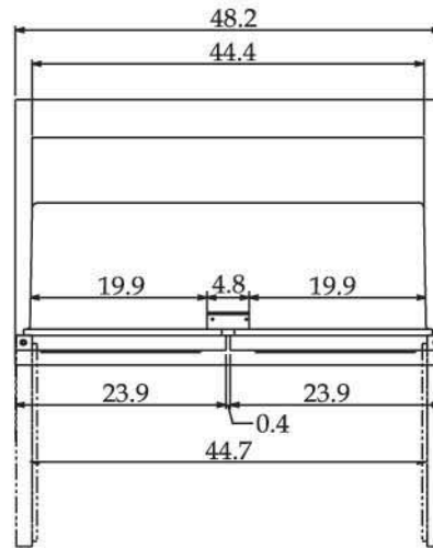
MUF-48 PLAN VIEW
