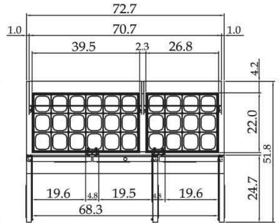
MST-72-30 PLAN VIEW
