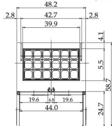
MST-48-18 PLAN VIEW
