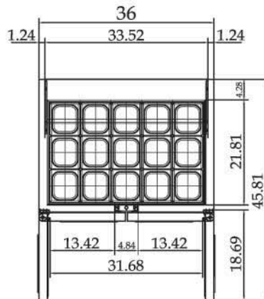
MST-36-15 PLAN VIEW
