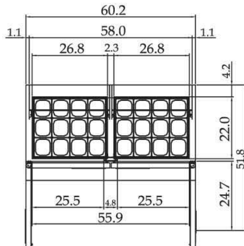
MST-60-24 PLAN VIEW
