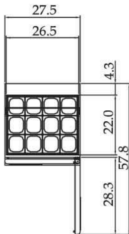
MST-28-12 PLAN VIEW
