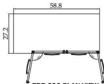
TBB-2SG PLAN VIEW
