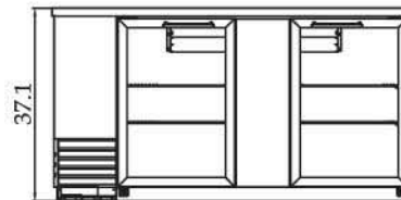
TBB-3SG FRONT VIEW
