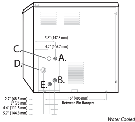
Water Cooled
