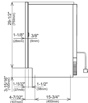
SIDE DIMENSIONS
