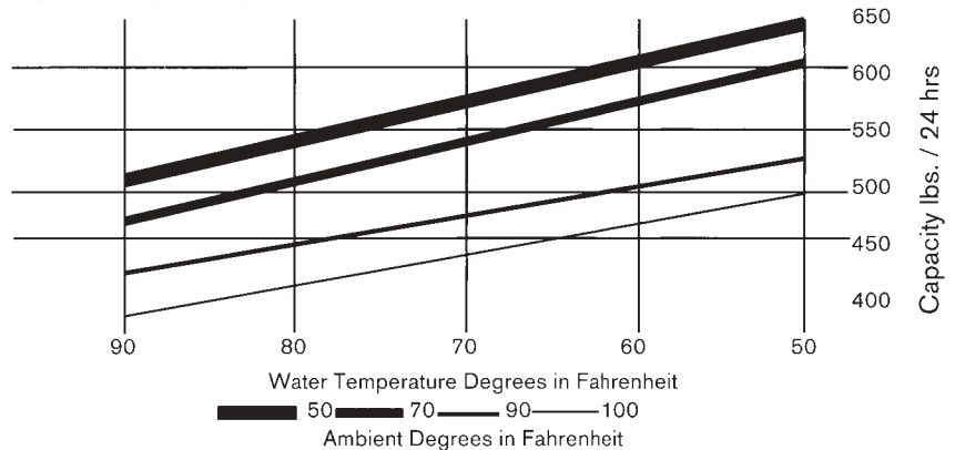
ICE MAKING CAPACITIES
