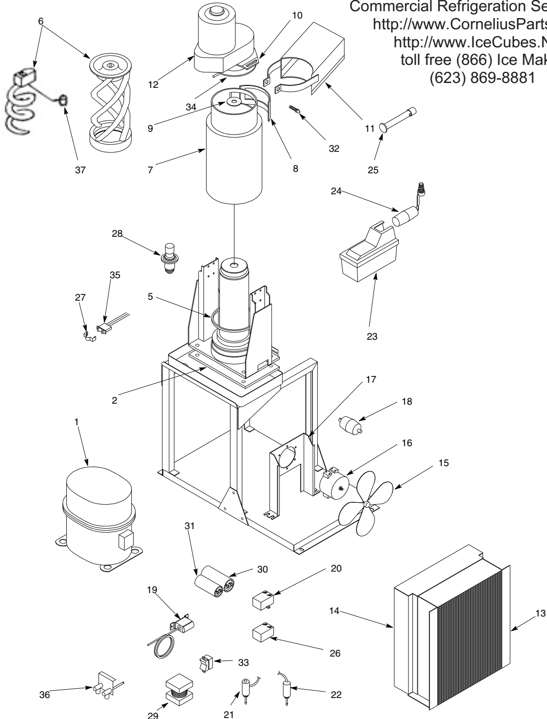
FIGURE 1. Exploded View
